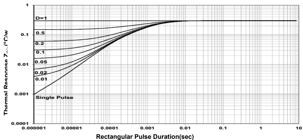
Fig. 19 Transient Thermal Impedance for IGBT
