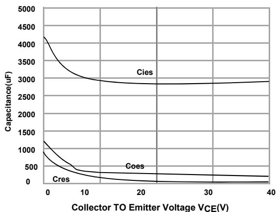
Fig. 5 Capacitance Characteristics
