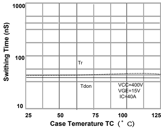
Fig. 11 T_C vs. Switching Loss
