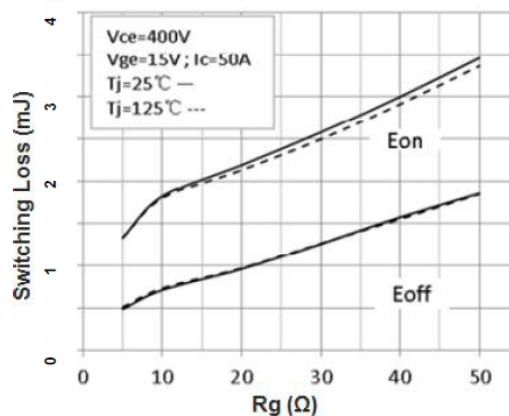
Fig. 6 Switching Energy Loss Characteristics
