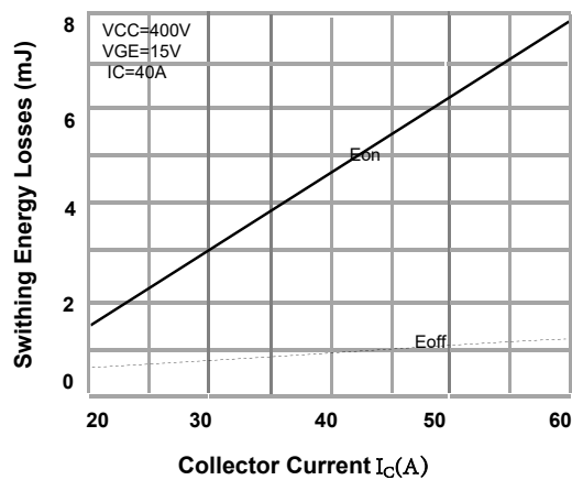
Fig. 12 I_C vs. Switching Loss
