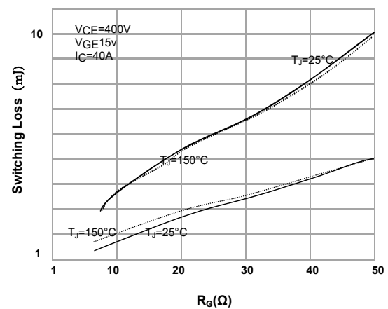
Fig. 6 Switching Energy Loss Characteristics
