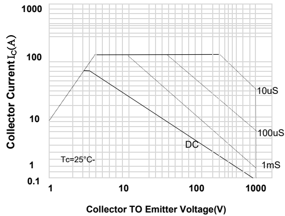
Fig. 14 Forward Safe Operating Area
