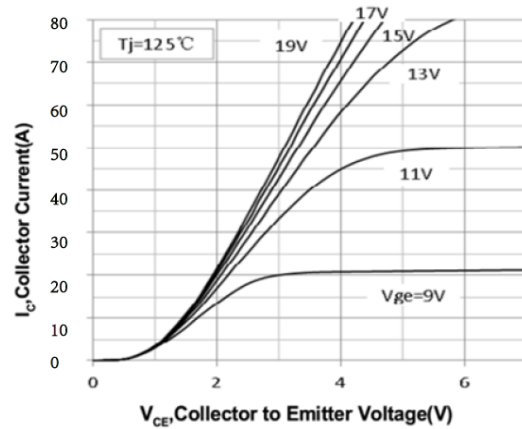
Fig. 2 Typical Output Characteristic
