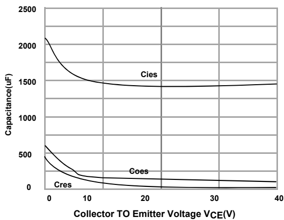
Fig. 5 Capacitance Characteristics
