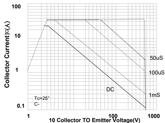
Fig. 13 Forward Safe Operating Area
