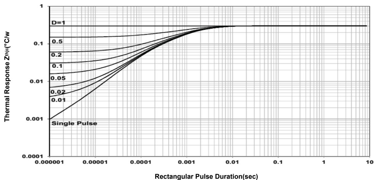
Fig. 14 Transient Thermal Impedance for IGBT
