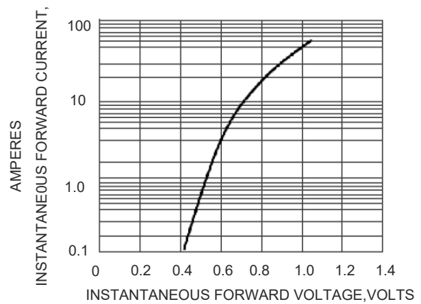
Fig. 4 Instantaneous Forward Characteristics
