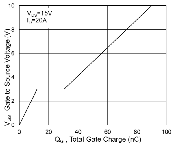
Fig.6 Gate-Charge Characteristics
