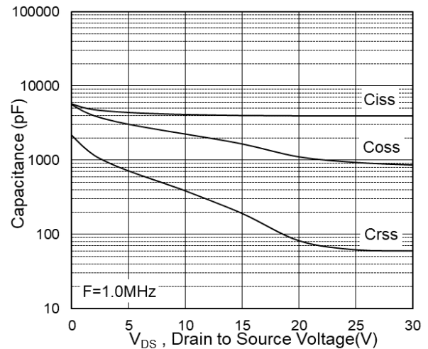
Fig.4 Capacitance
